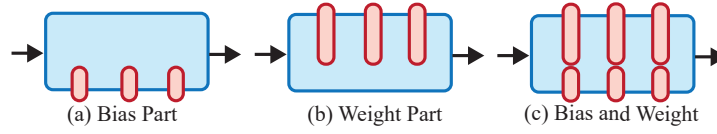
Fig. 4. Three types of parameter tuning. Red and blue parts are tunable and frozen parameters, respectively.
