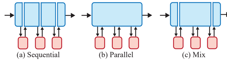
Fig. 3. Three different types of adapter methods. Red and blue parts are tunable and frozen parameters, respectively.
